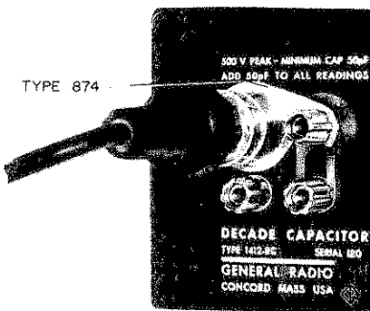
Figure 4. Type 1412-BC showing two-terminal (grounded) connection using Type 874
